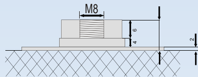
T11 Threaded Insert 8mm Stud
